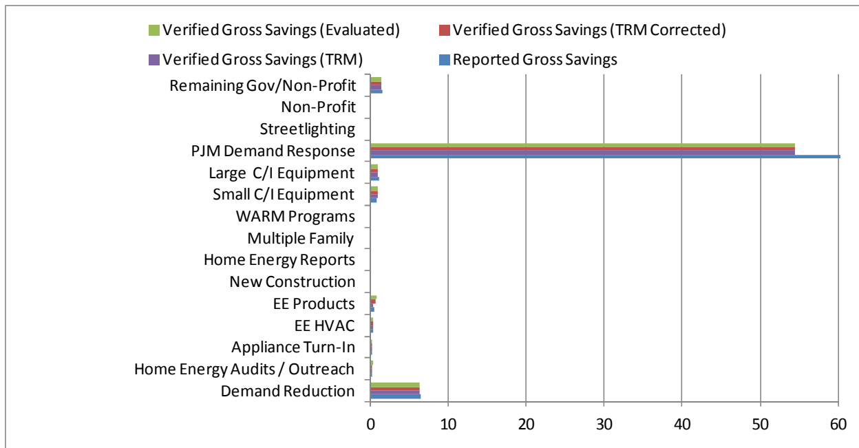
Figure 1-7: PYTD Reported Demand Reduction by Program (Top 100 Hours)
