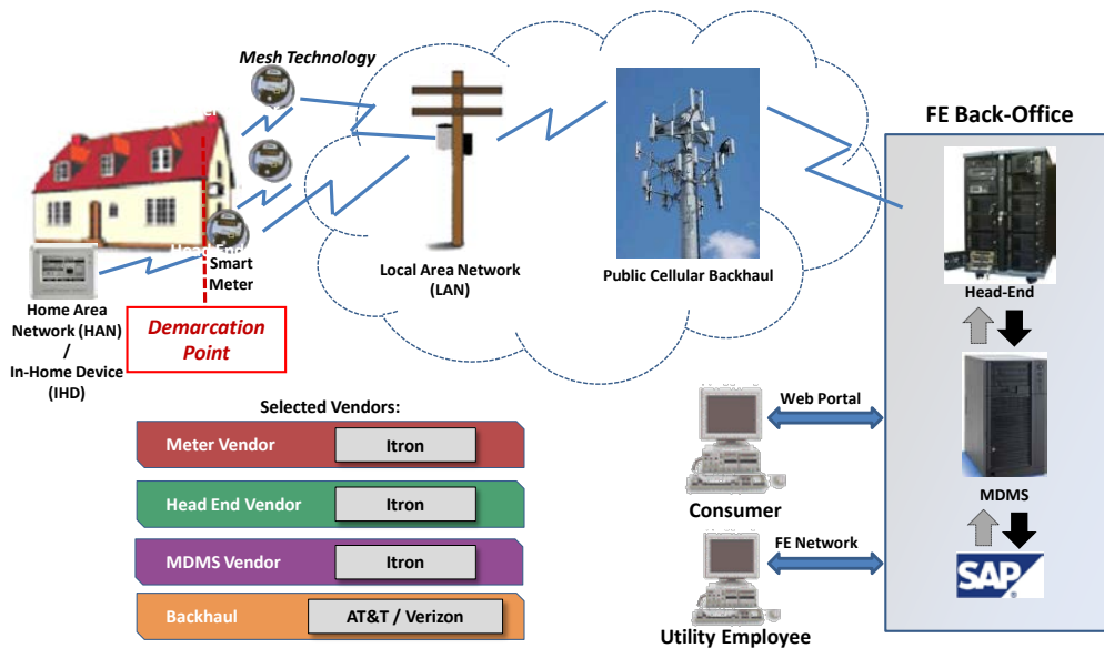
Figure 3.1 PA Companies Smart Meter Solution
