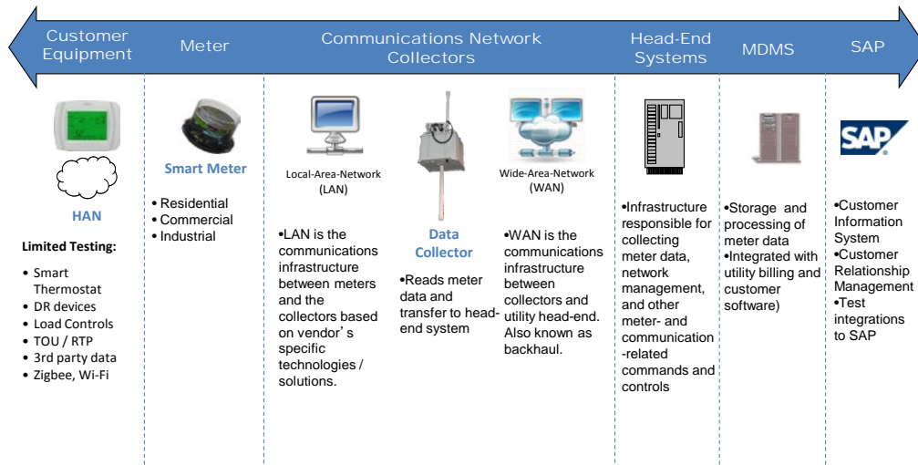
Figure 2.1 AMI High Level Scope Overview
